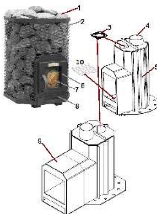
Figure 1. Heater components
